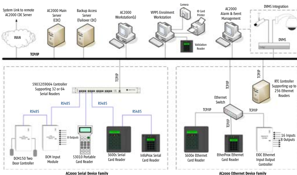
AC2000 AE System Topology
